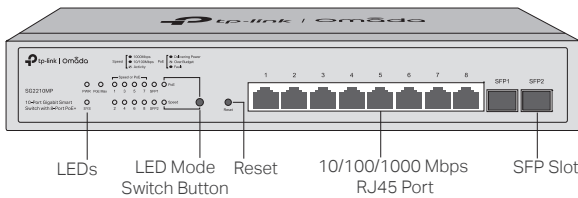
Figure 1-2 Front Panel of SG2210MP
