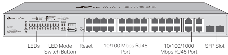
Figure 1-6 Front Panel of SL2428P
